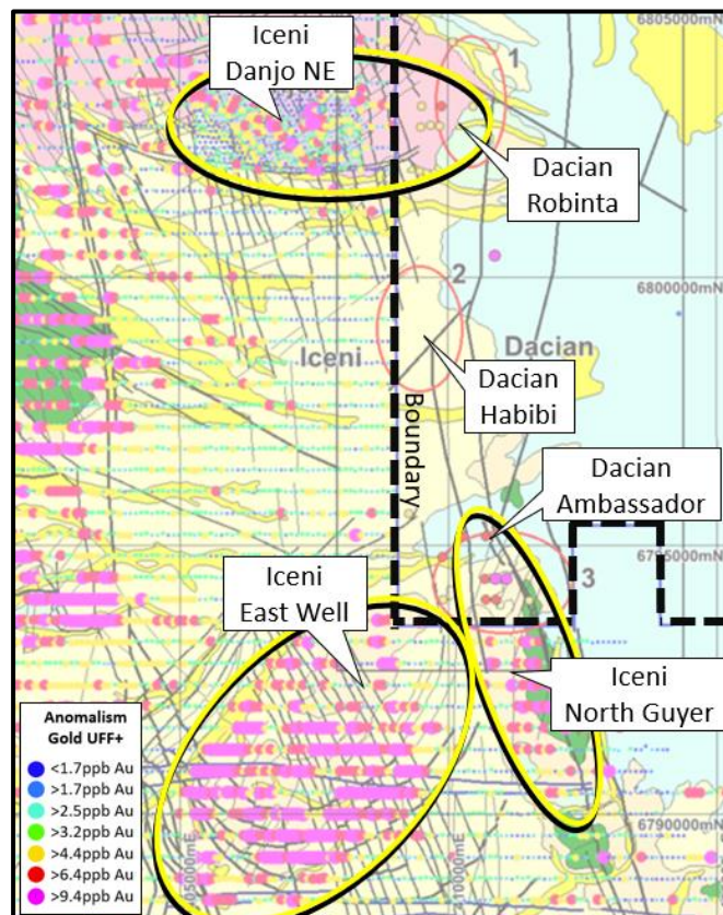
Figure 1: Gold anomalies identified in UFF results extend over the Iceni 14 Mile Well Project boundary into ground operated by Dacian Gold Ltd.
