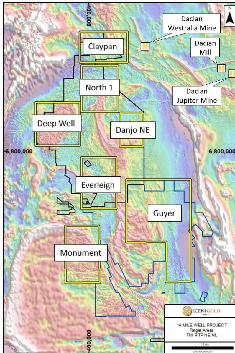
Figure 3: 14 Mile Well Project area, showing the seven key target areas relative to neighbouring infrastructure. Gold anomalies extend from the Danjo NE and Guyer target areas onto ground operated by Dacian Gold Ltd.
